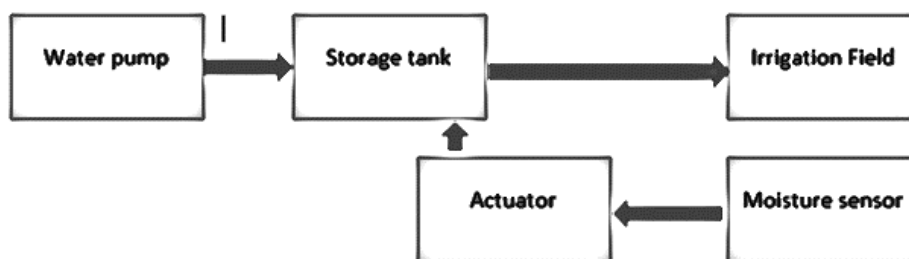
Figure 3.2.Automatic Irrigation Module Block Diagram
